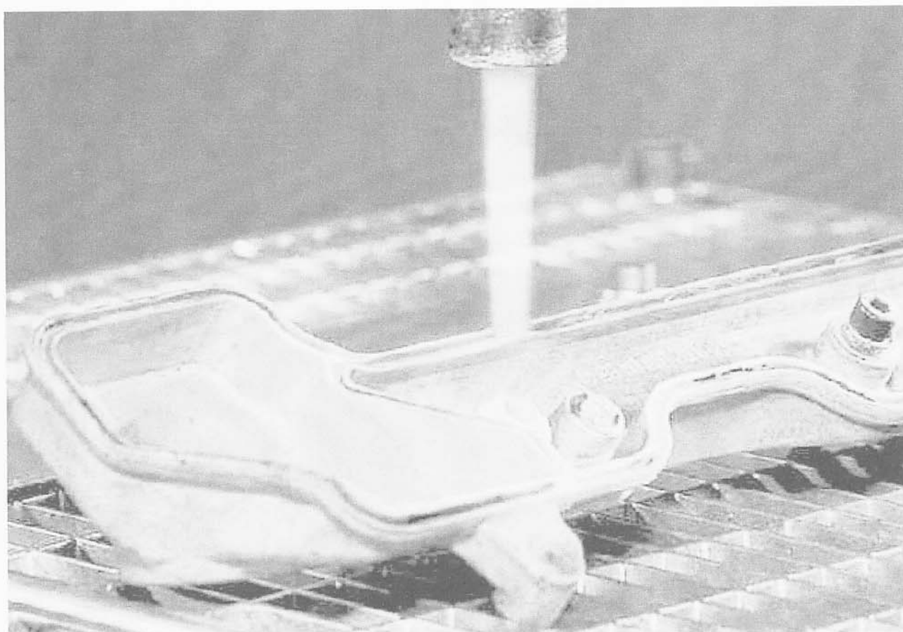
Figure 6: Removing silicone seals from valve bonnet of the of Mercedes-Benz A-class
