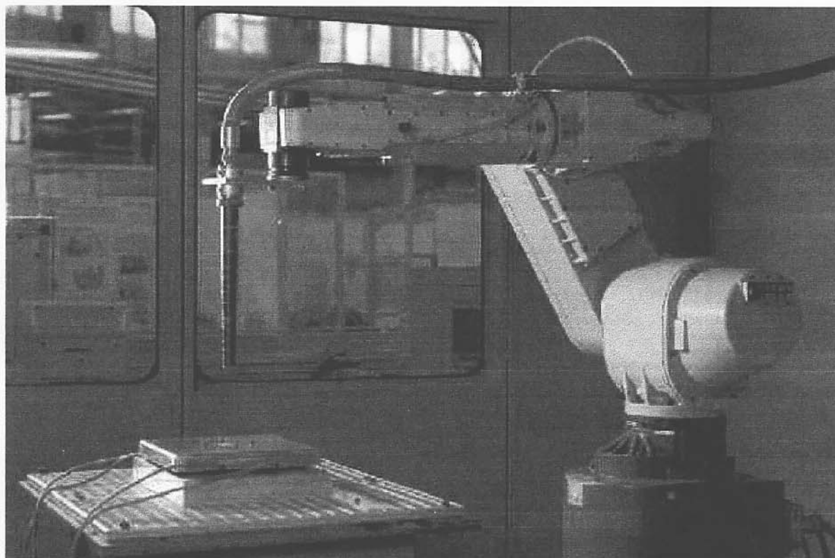
Figure 5: 6-axes-robot for blasting operation
