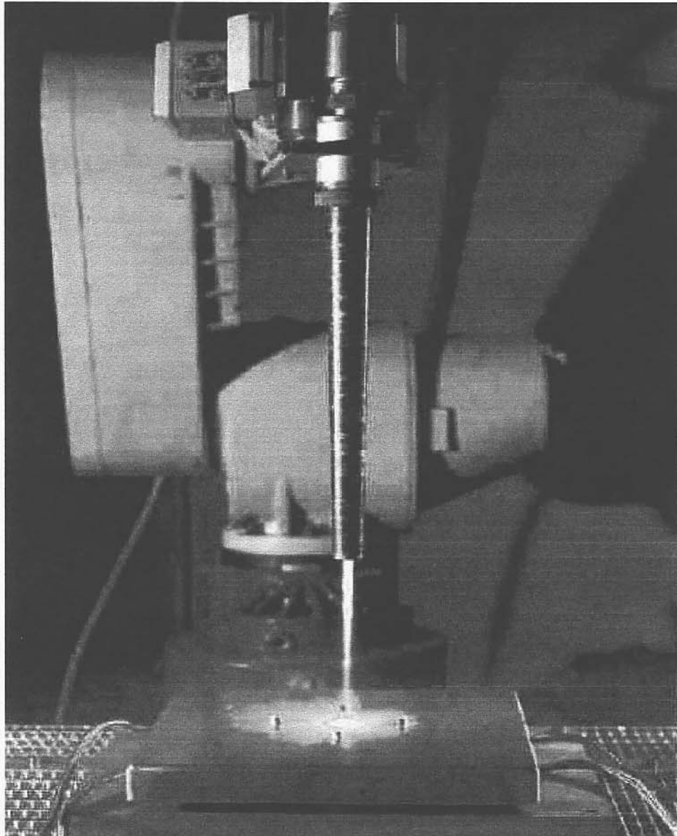
Figure 2: Force measurement in dry-ice blasting
