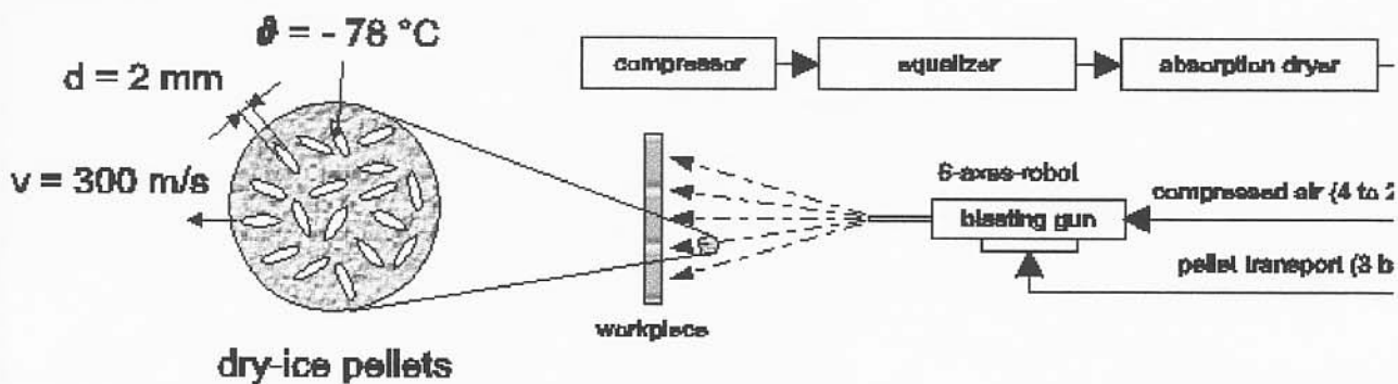
Figure 1: Process principle of dry-ice blasting
