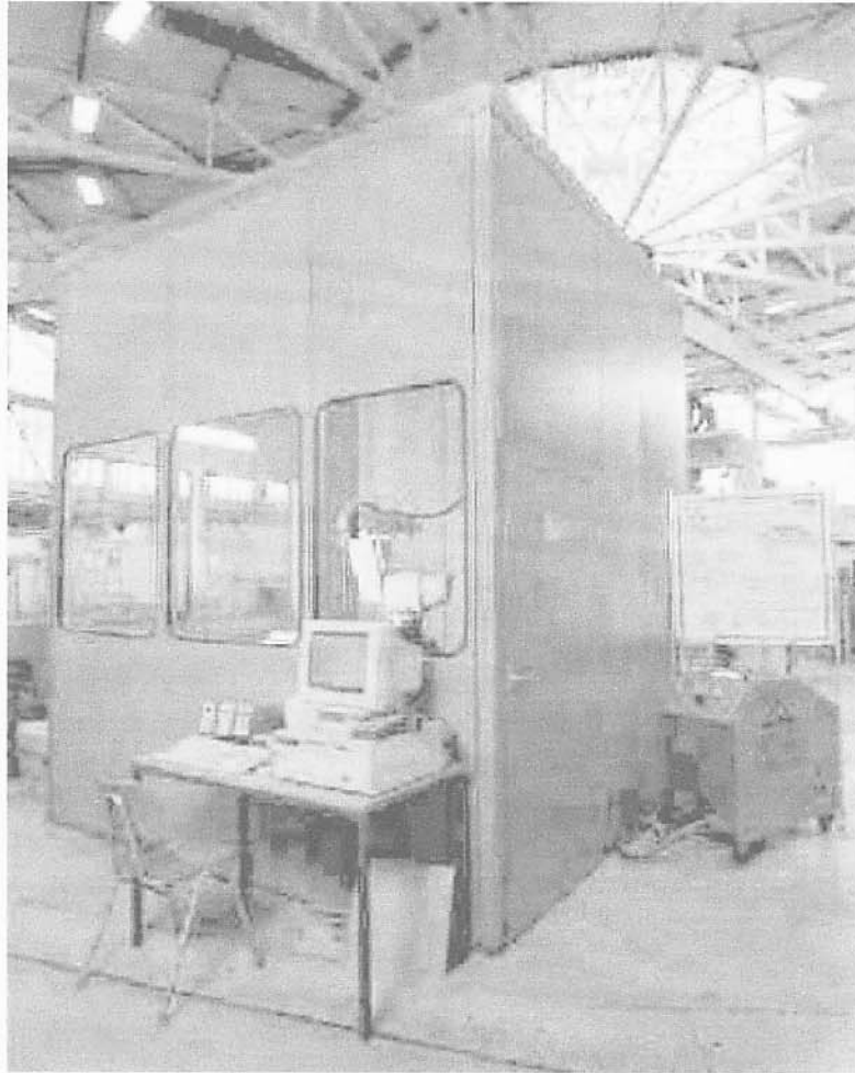
Figure 4: Test stand for dry ice blasting at the Institute for Machine Tools and Factory Management
